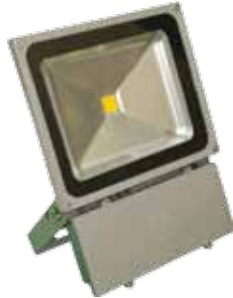
Veto LED FLOOD LIGHT 100W D/L 100% HEAVY DUTY. Available in 10W, 20W, 30W, 50W, 70W, 100W, 150W, 200W ITEM CODE : VELFL100A
