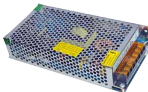
Veto LED TRANSFORMER 10A/175W Available in 2A/35W, 5A/87.5W, 10A/175W ITEM CODE : VELT10A
